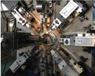
C&C Spring manufacturing machine
